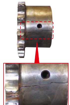
Example of fracture due to insufficient hub strength
